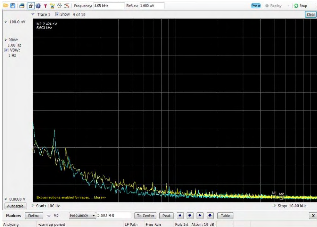
Figure 22: Noise Density 100nV full scale, mid range noise density is 2nV/Root-Hz.
