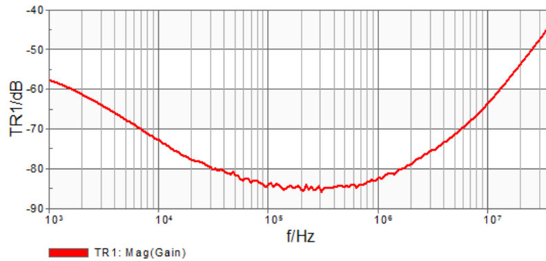
Figure 26: Frequency response of the J2102A.
