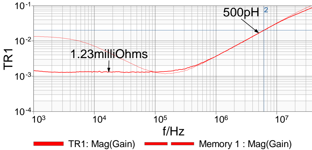
Figure 27: Impedance measurement of a 1\text{m}\Omega resistor with and without the J2102A common mode transformer using the OMICRON Lab Bode 100.
