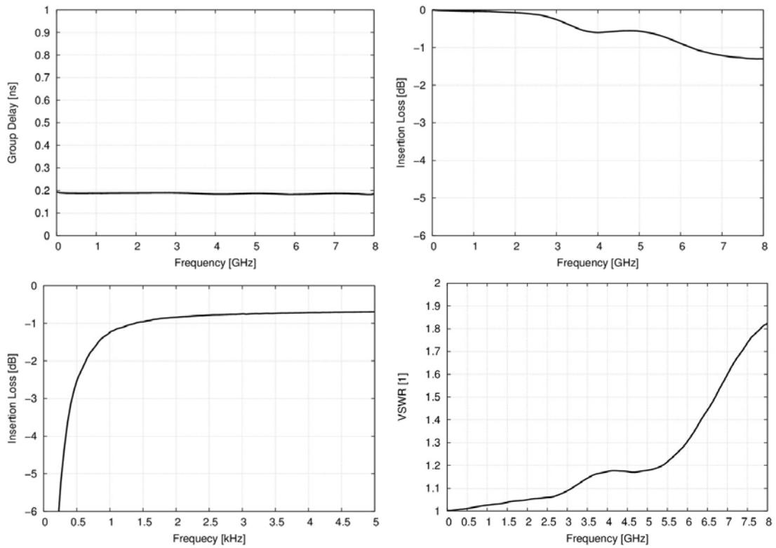
Figure 16: Electrical performance characteristics of the P2130A DC blocker.
