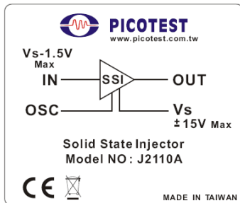
Figure 8 Solid State Injector Connections for stability measurements.
