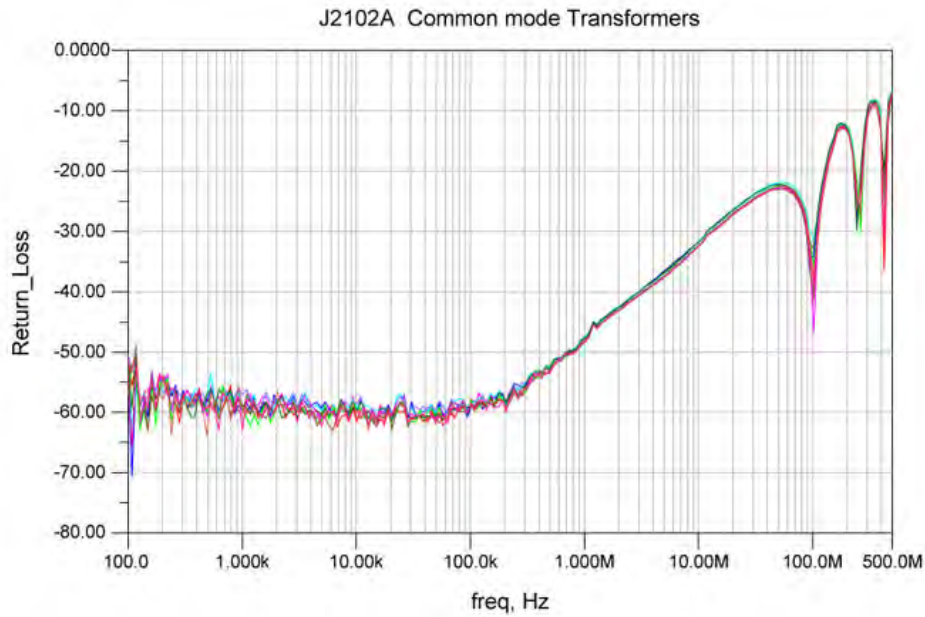
Figure 29: J2102A Return Loss Graph.
