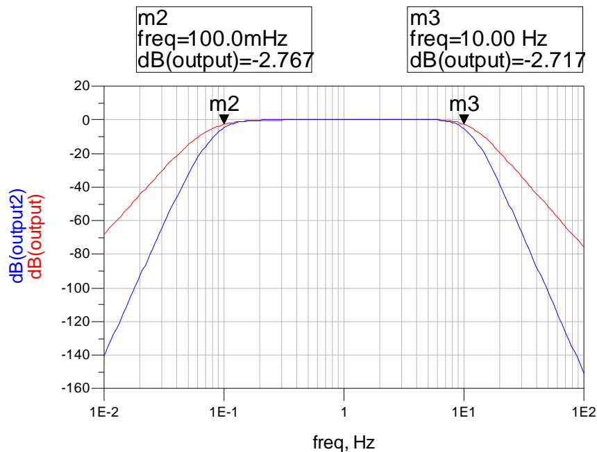
Figure 23: Frequency response of a single filter (red trace) and 2 cascaded filters (blue trace).
