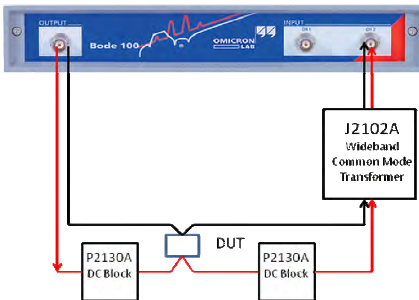
Figure 24: Connection diagram showing the placement of the J2102A common mode transformer. Inclusion of the transformer eliminates the low frequency distortion caused by
