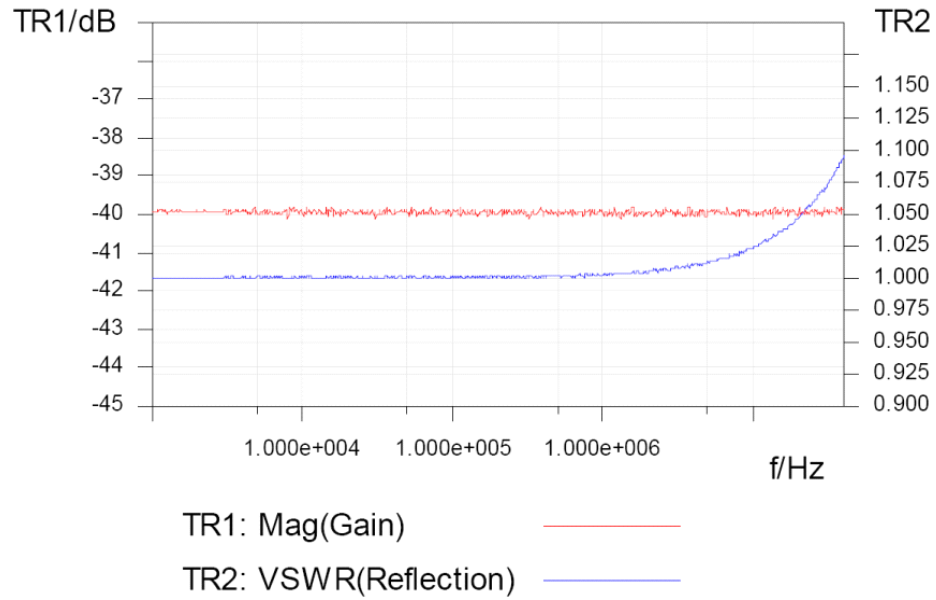
Figure 20: 40dB attenuator frequency response.
