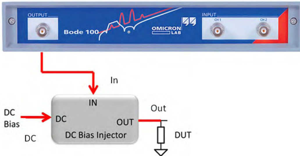
Figure 13: Connections for DC Bias Impedance measurements.
