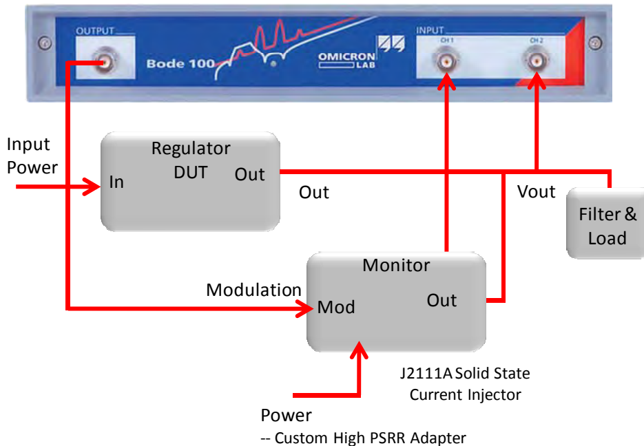
Figure 18: Current Injector Connections for output impedance measurements.
