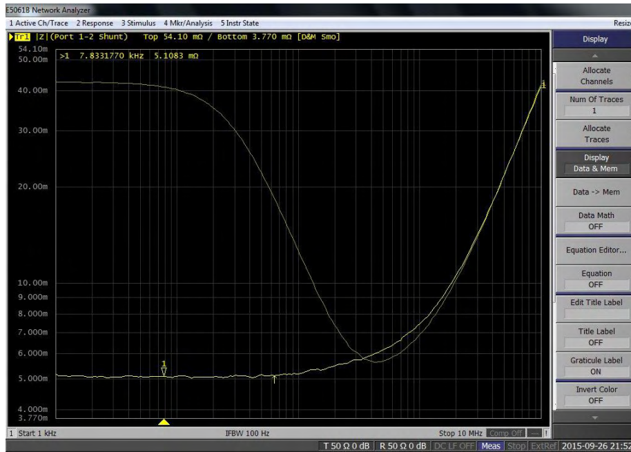
Figure 28: Impedance measurement of a 5\text{m}\Omega resistor with and without the J2102A common mode transformer using the Keysight E5061B.
