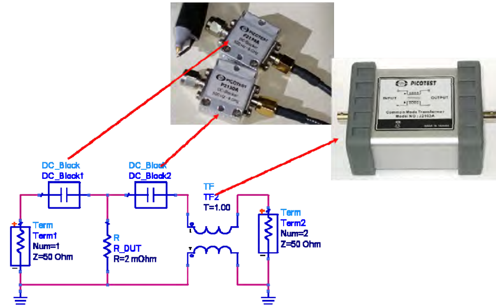
Figure 25: Electrical connection diagram showing the placement of the J2102A and P2130A DC blockers for a 2 port shunt impedance measurement.
