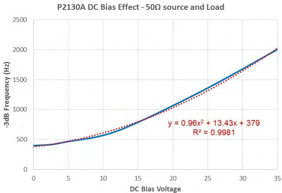
Figure 15: The effect of DC bias on the P2130A DC blocker frequency performance which shifts the - 3dB frequency.
