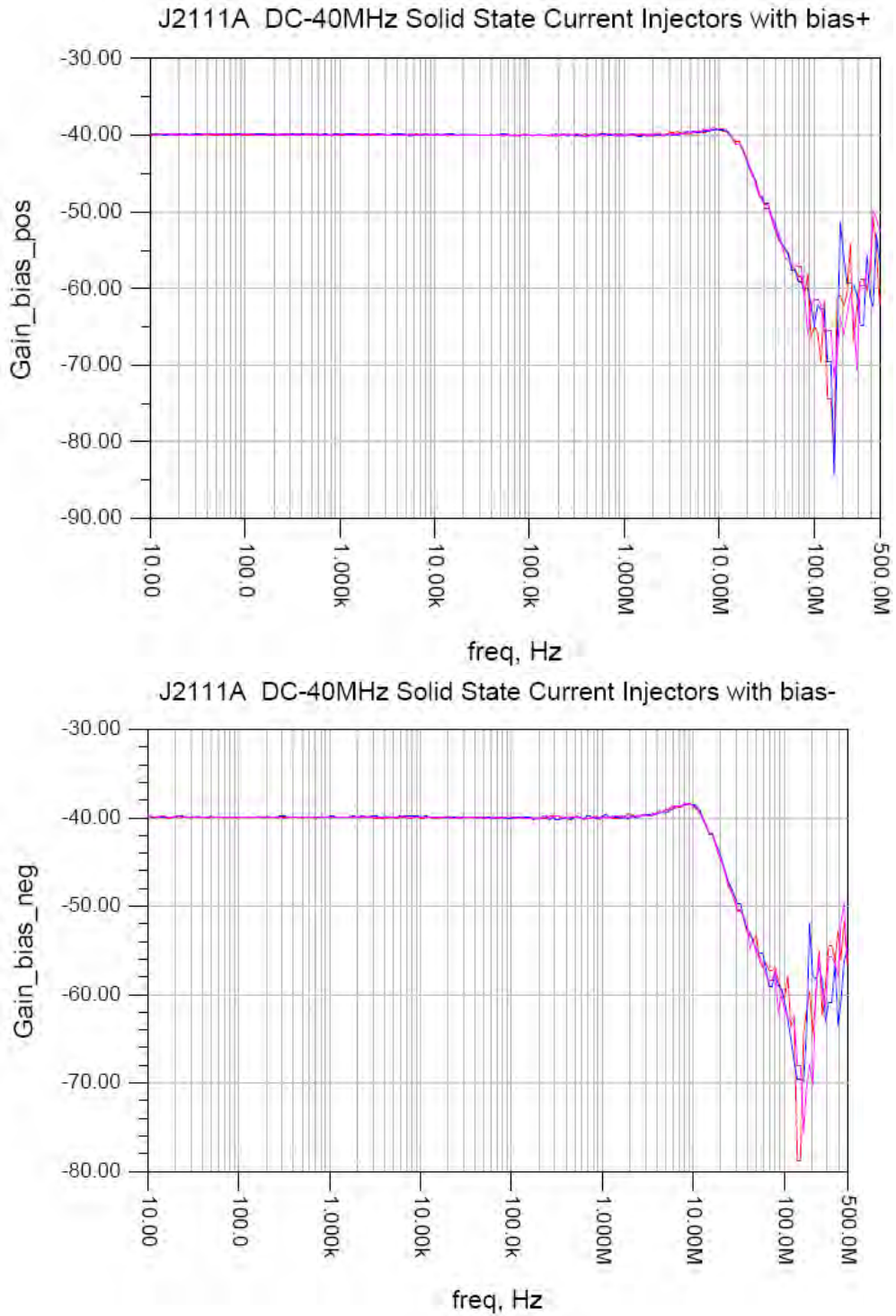
Figure 19: J2111A frequency response.
