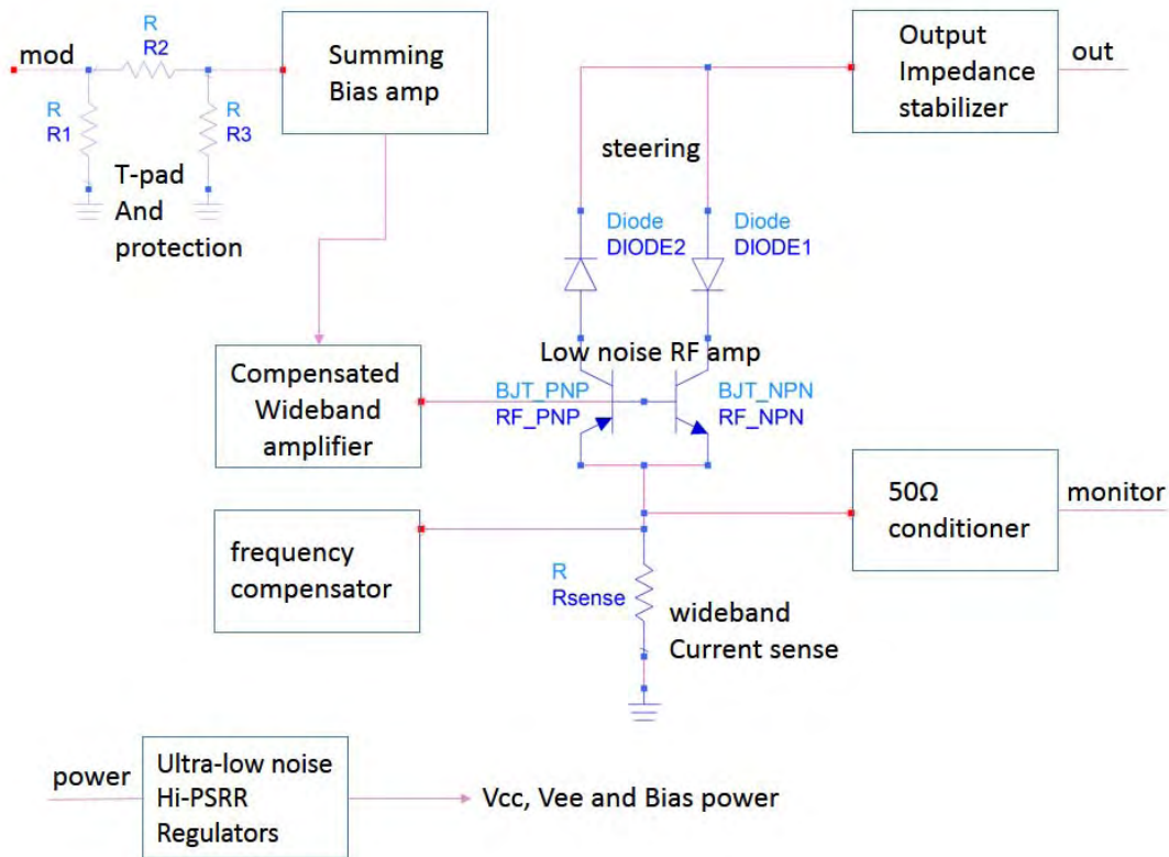
Figure 17: Current Injector internal block diagram.
