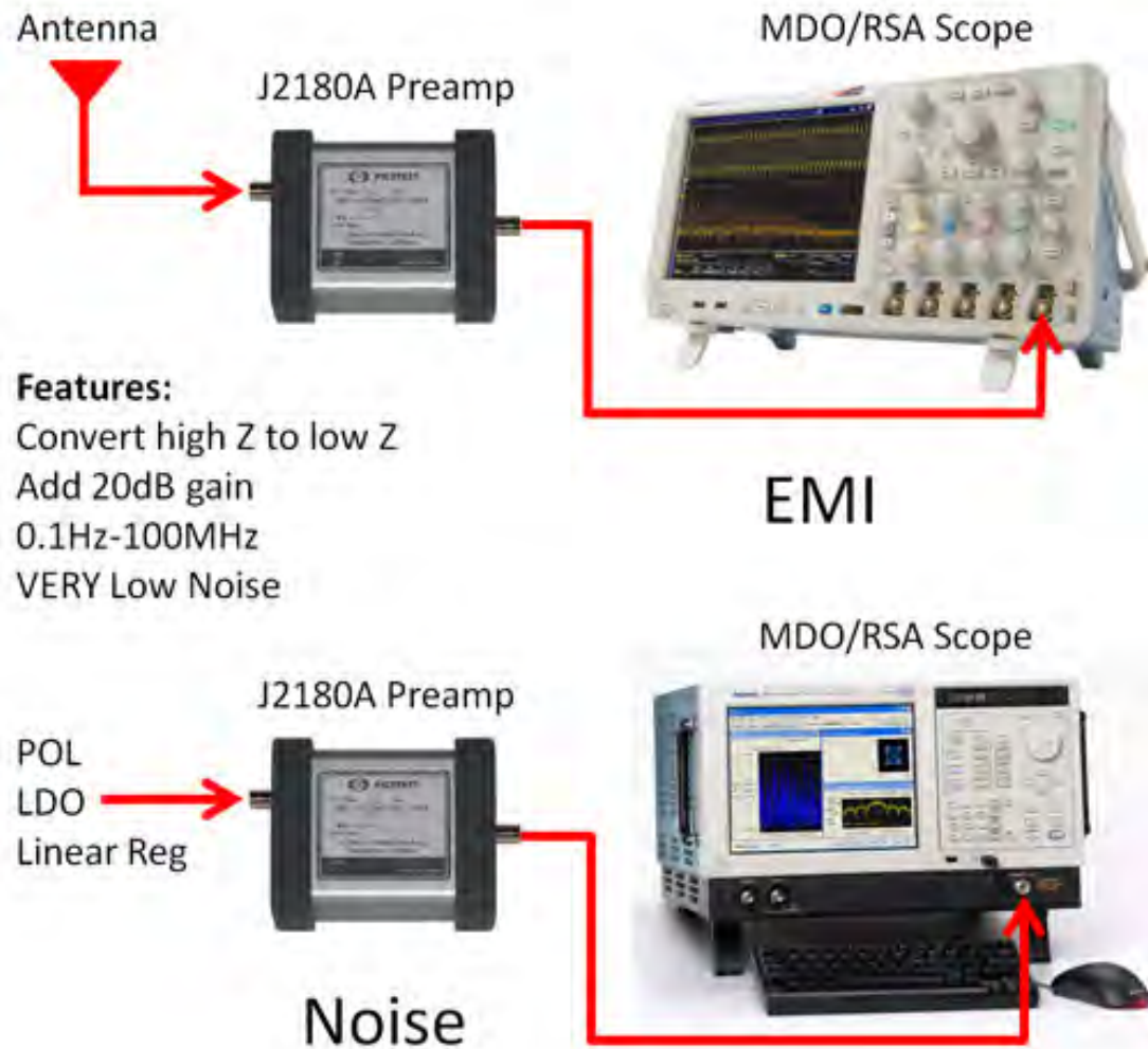
Figure 21: Sample setups for the J2180A Preamp used for noise and EMI measurements.
