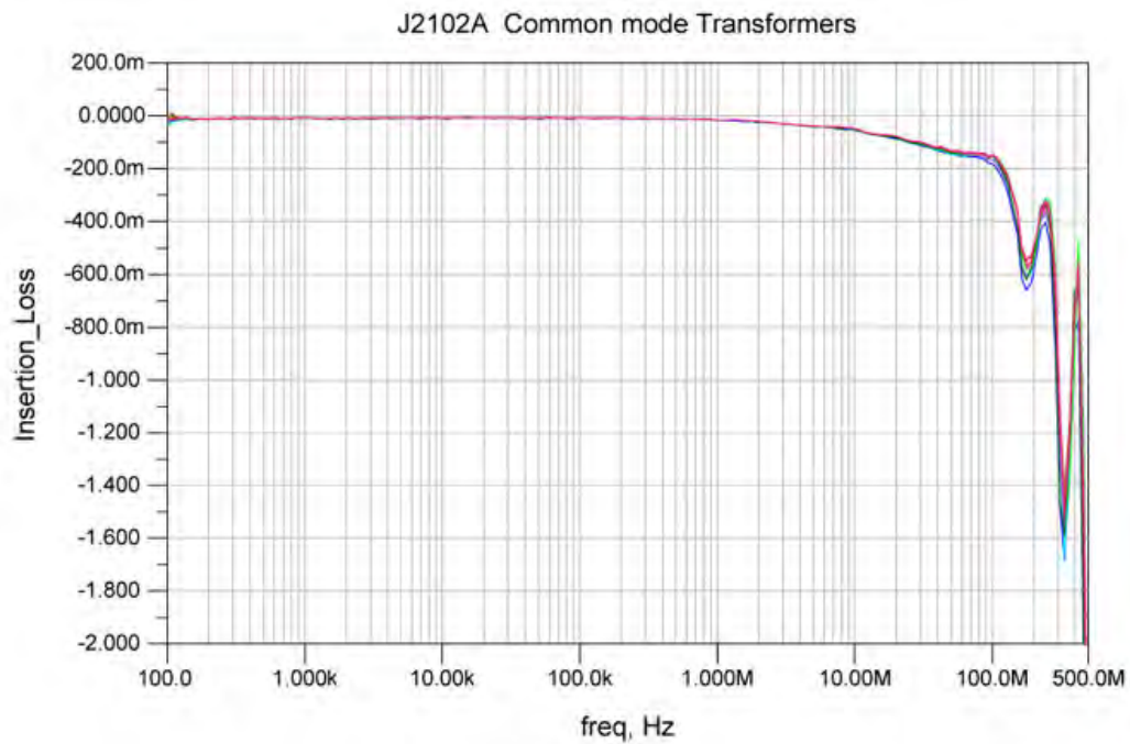
Figure 30: J2102A Insertion Loss Graph.
